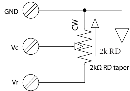
VR1 Block Diagram and Schematic
