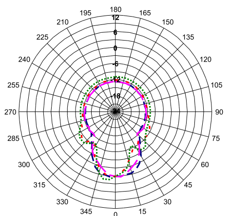
Horizontal coverage
