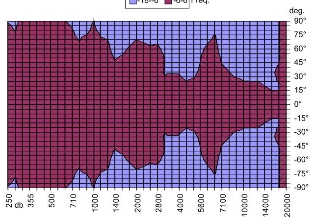
Horizontal coverage
