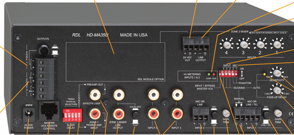
OUTPUT DETAIL HD-MA35U
