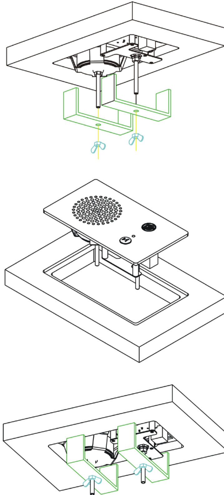
Figure 3.3.8 Installation of HCS-48U7MICSPK series flush-mounted congress unit
