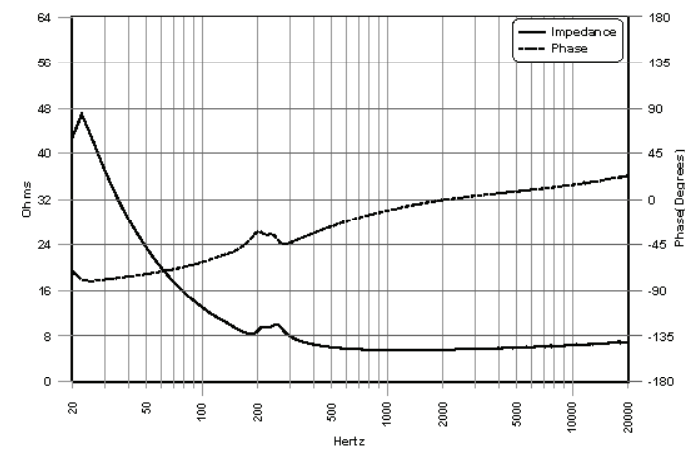
Phase/Impedance Response
