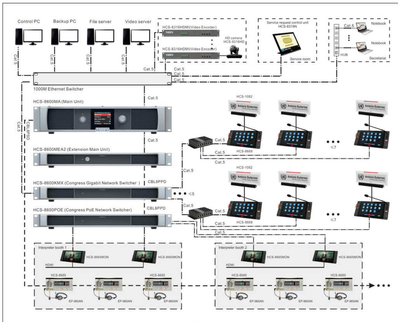
Figure 1.1.5 HCS-8668 Series Paperless Multimedia Congress System connection diagram (POE)
