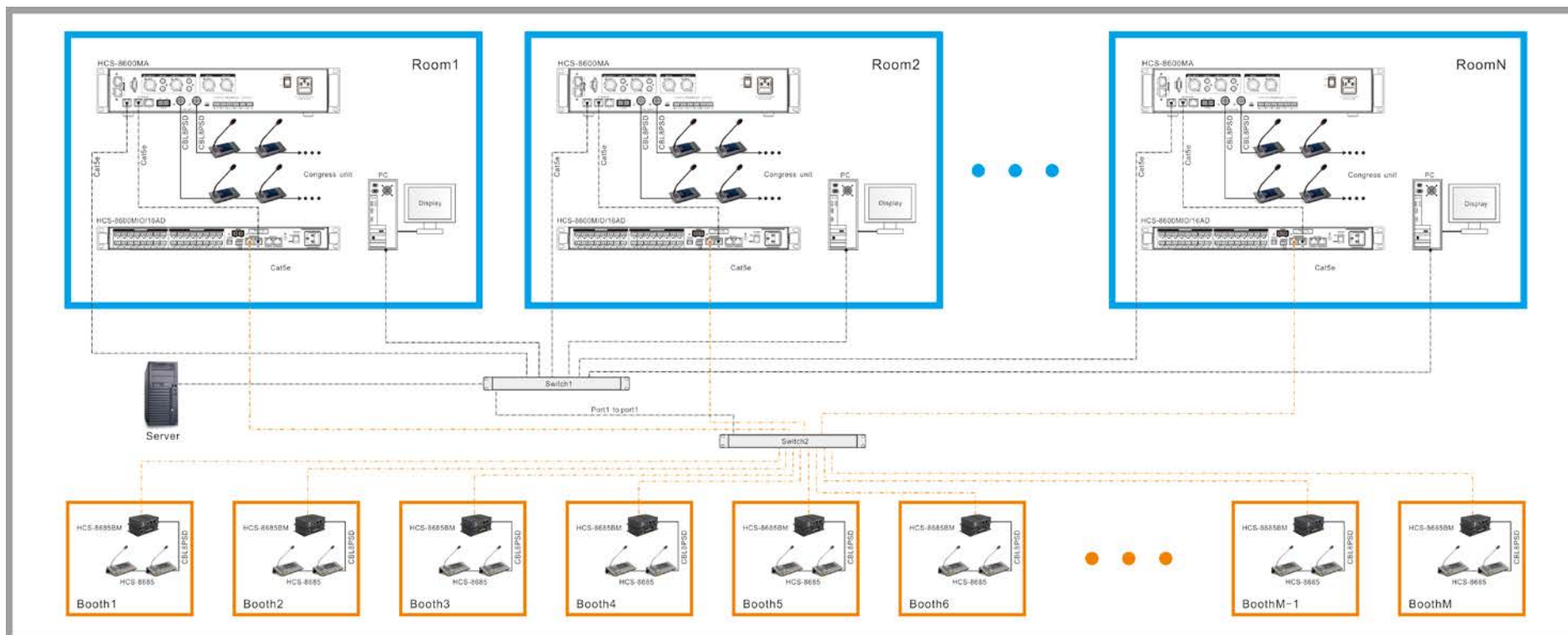
Figure 6.5.2-1: Connection diagram of booth management system
