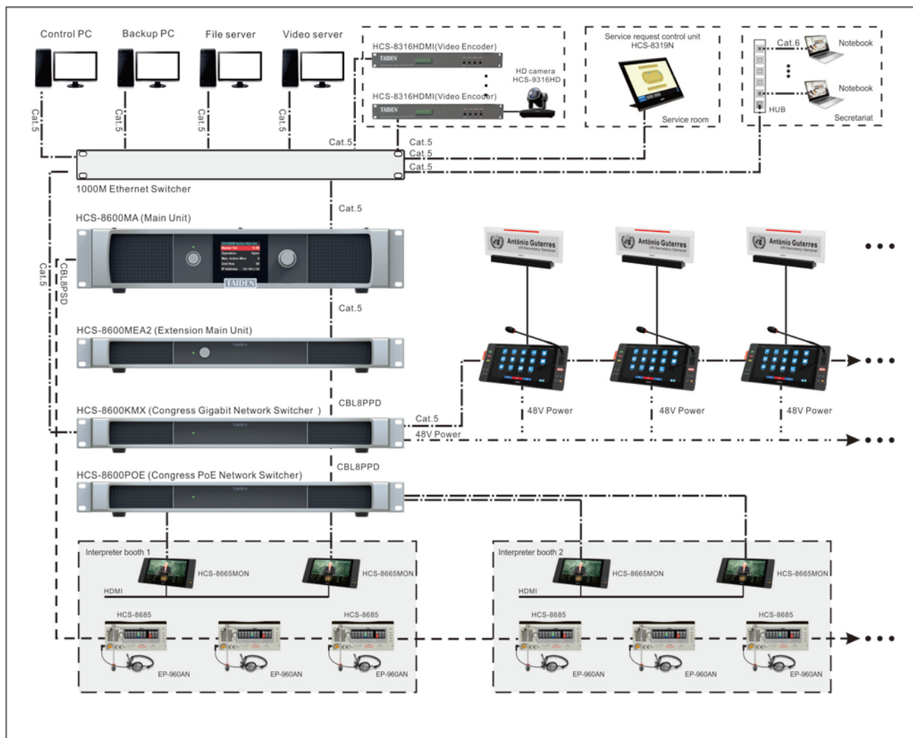
Figure 1.1.4 HCS-8668 Series Paperless Multimedia Congress System connection diagram
