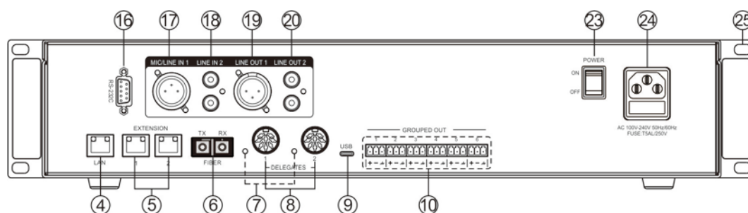
Backside of HCS-8600M CMU
