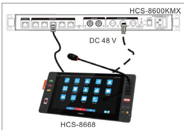
Figure 3.2.6 HCS-8668/8638 series paperless multimedia congress terminal connecting to HCS-8600KMX Ethernet switch (not PoE)
