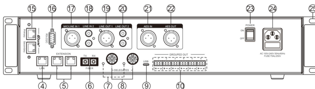
Backside of HCS-8600MA CMU
