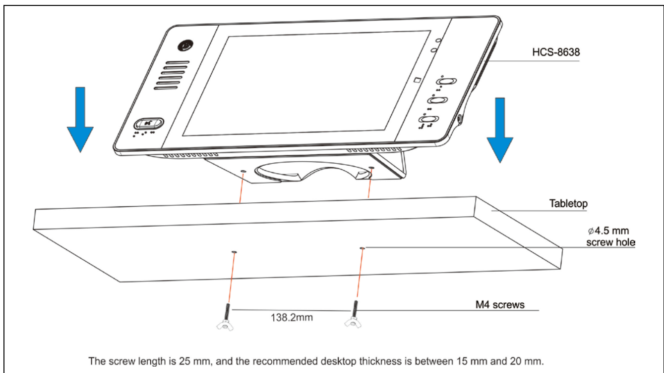
Figure 3.2.4 Fixed installation of HCS-8638/50 series congress unit
