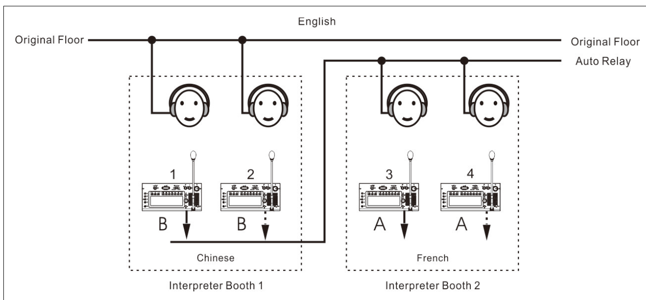
Figure 4.8 Relay interpretation
