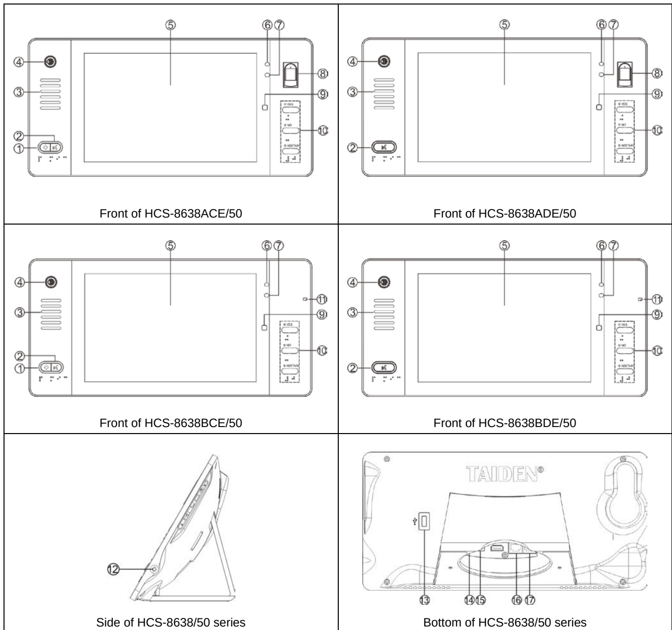
Figure 3.2.2 HCS-8638/50 series Paperless Multimedia Congress Terminal
