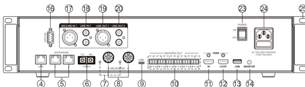
Backside of HCS-8600MBU CMU
