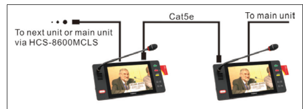
Figure 3.4.5 "Daisy-chain" connection between HCS-8635 series compact multimedia terminals
