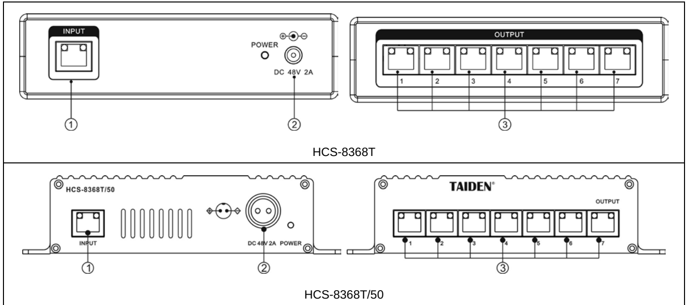
Figure 6.4.1 HCS-8368T Distributor
