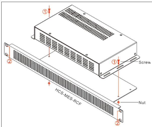
Figure 2.3.2 Cabinet installation of HCS-8600MES
