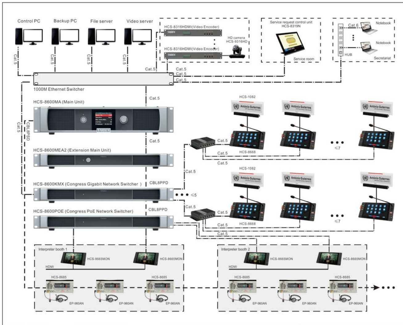
Figure 6.2.3 HCS-8668 Series Paperless Multimedia Congress System connection diagram (POE)
