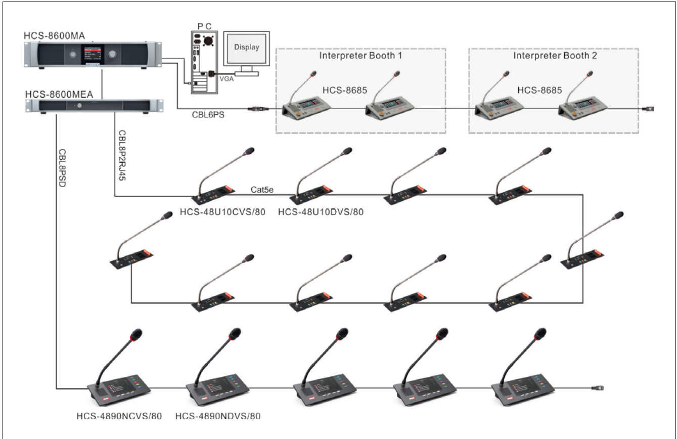
Figure 5.2.1 Connection example of HCS-8600 series congress system
