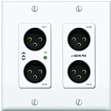
unDX4I Front Panel
