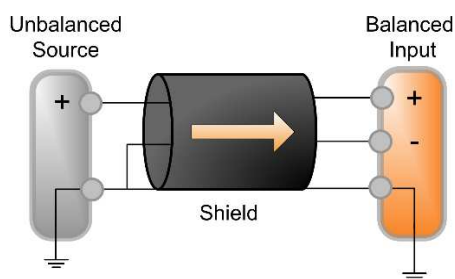
Figure 4 - 2-Wire Unbalanced Source Connection
