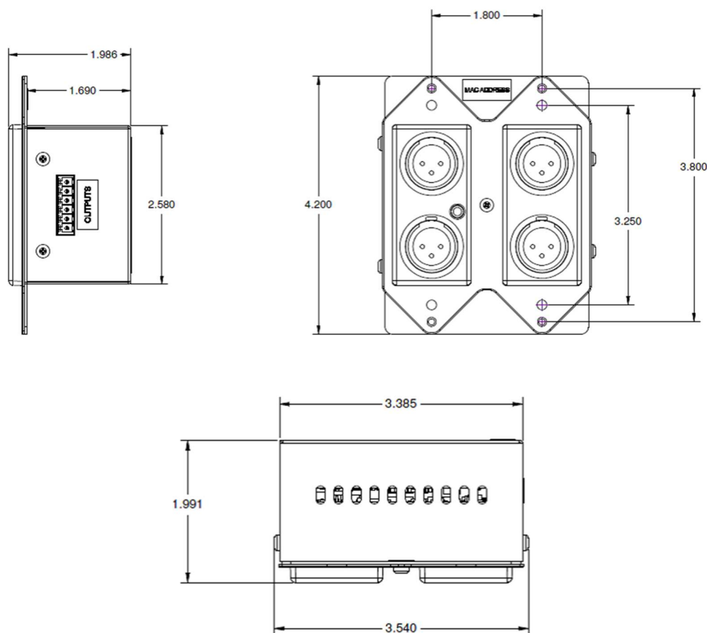
Figure 3 - Mounting Information
