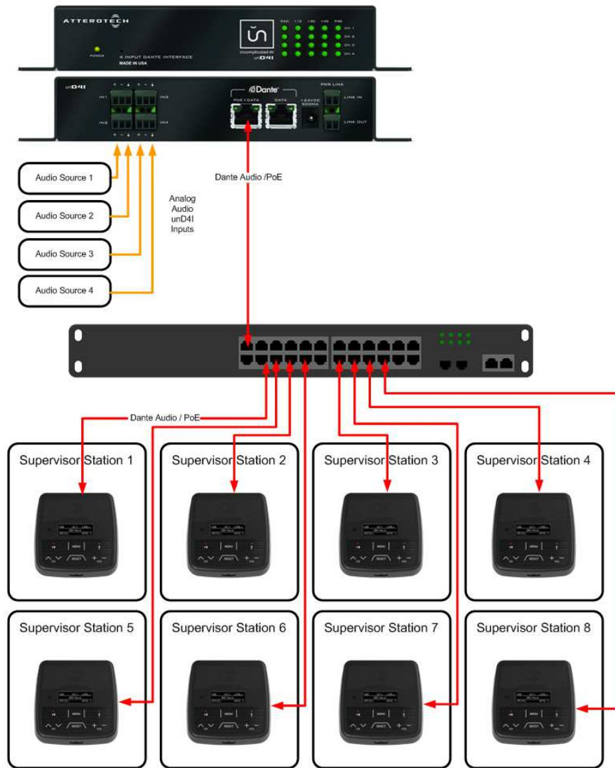
Figure 18 - PoE Deployment
