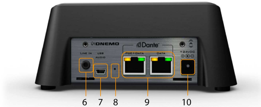
Figure 2 - unDNEMO Rear Panel Features
